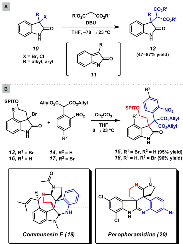
Scheme 1. Alkylations of 3-Halooxindoles
