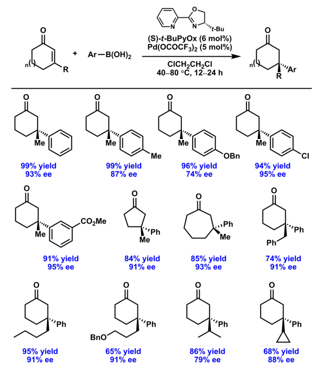
Scheme 3. Large Scale Conjugate Additions
