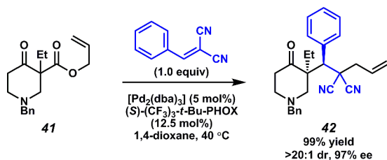
Scheme 11. Asymmetric Enolate Alkylation Cascade with Different Electrophiles
