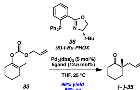
Scheme 8. Discovery of an Enantioselective Catalyst System for the Asymmetric Tsuji Allylic Alkylation
