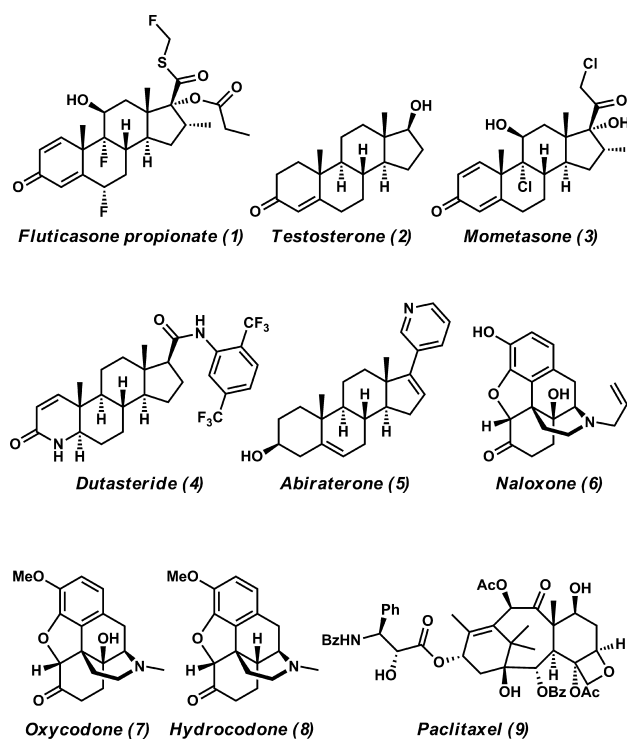
Figure 1. Drug molecules containing quaternary stereocenters.
