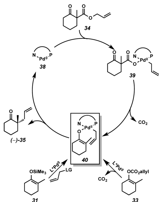
Scheme 10. Generation of Palladium Enolate Intermediates from Other Starting Materials
