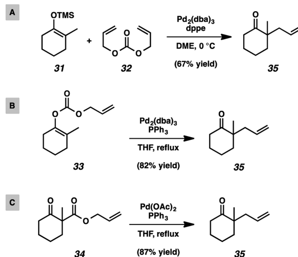
Scheme 8. Discovery of an Enantioselective Catalyst System for the Asymmetric Tsuji Allylic Alkylation
