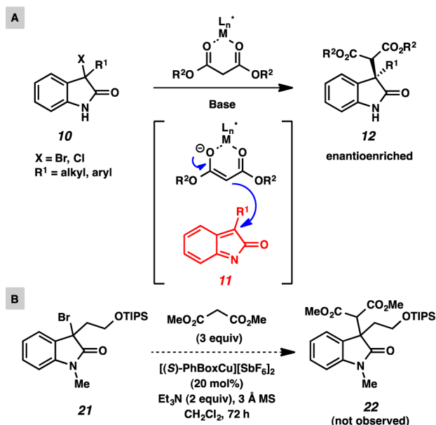
Scheme 2. Alkylations of 3-Halooxindoles via Reactive Prochiral Indolone 11
