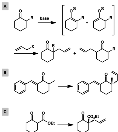
Scheme 6. Challenges in Alkylation of Nonsymmetrical Ketones
