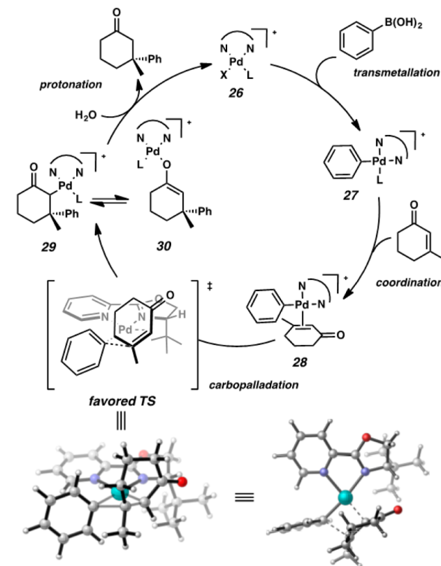
Scheme 4. Mechanistic Rationale for the Asymmetric Conjugate Addition
