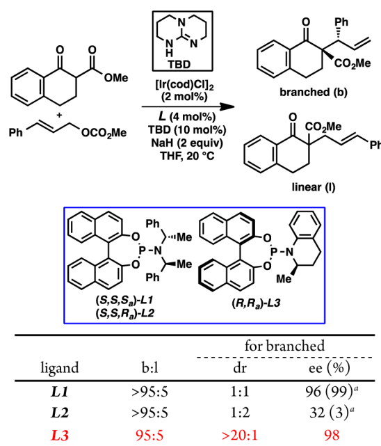
Scheme 12. Ir-Catalyzed Allylic Alkylation of Cyclic \alpha -Substituted \beta -Ketoesters
