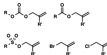
Figure 2. Substrate possibilities for the enantioselective alkylation reaction.
