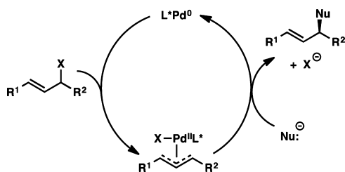
Scheme 6. Challenges in Alkylation of Nonsymmetrical Ketones
