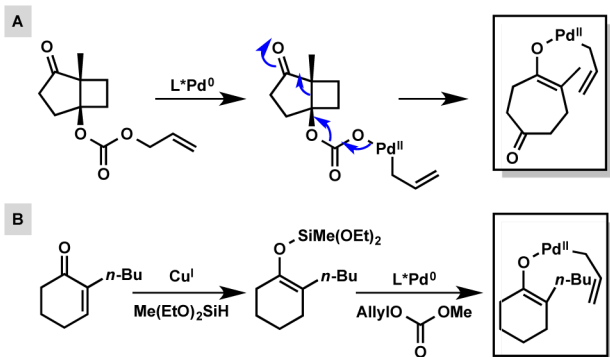
Scheme 11. Asymmetric Enolate Alkylation Cascade with Different Electrophiles
